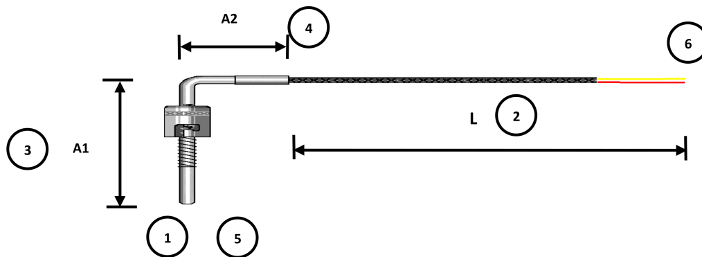
RIGHT ANGLE TUBE & WIRE SENSOR
