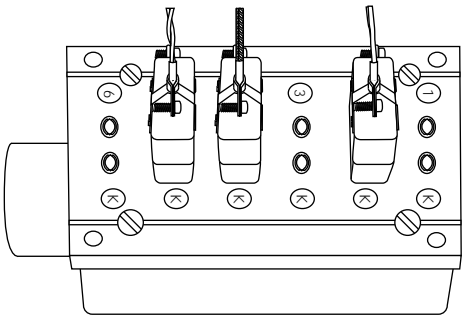
940 multi-circuit jack panel mounted in 942 FS box. Nominal dimensions: 940 panel 4 3/4 in X 2 3/4 in X 1 in, 942 box 4 3/4 in X 2 13/16 in X 2 1/16 in.
